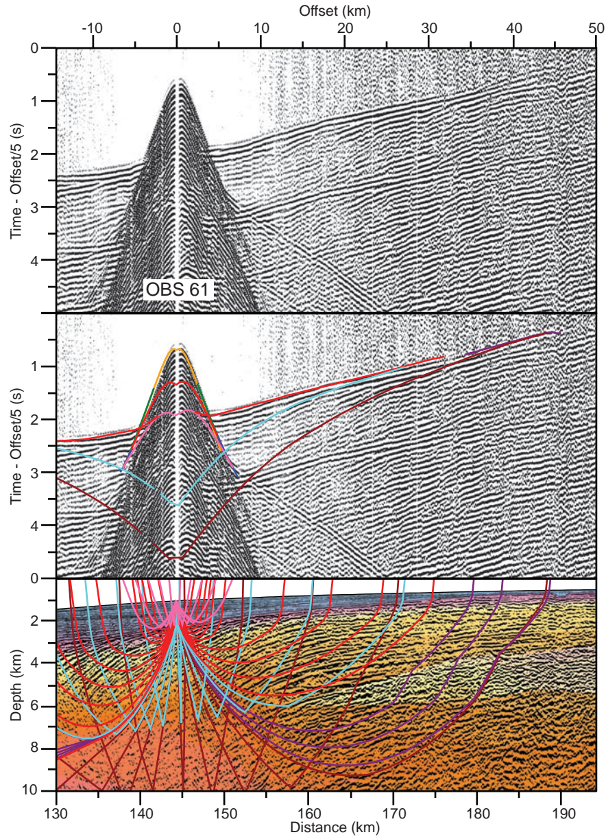
Fig S18. (Top) Record section for geophone data of OBS 61. A linear moveout at 5 km/s has been applied. Distances are measured from the north-northwestern end of the complete model (as in Roberts et al. 2009) and offsets are shot-receiver distances. (Middle) Record section with traveltime curves calculated by raytracing through the final velocity model and colour-coded by phases (see Figure 4 for legend). (Bottom) the corresponding ray path diagram with the same colour code as above. Only top basalt and deeper phases are shown for clarity. The seismic section was prestack depth migrated using the same final P-wave velocity model (colourmap) as is used in the raytracing. See text for modelling details. See Figure 8 in main paper for OBS location.
